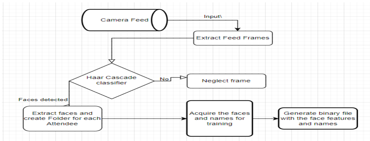
Fig. 1. The workflow of the module
