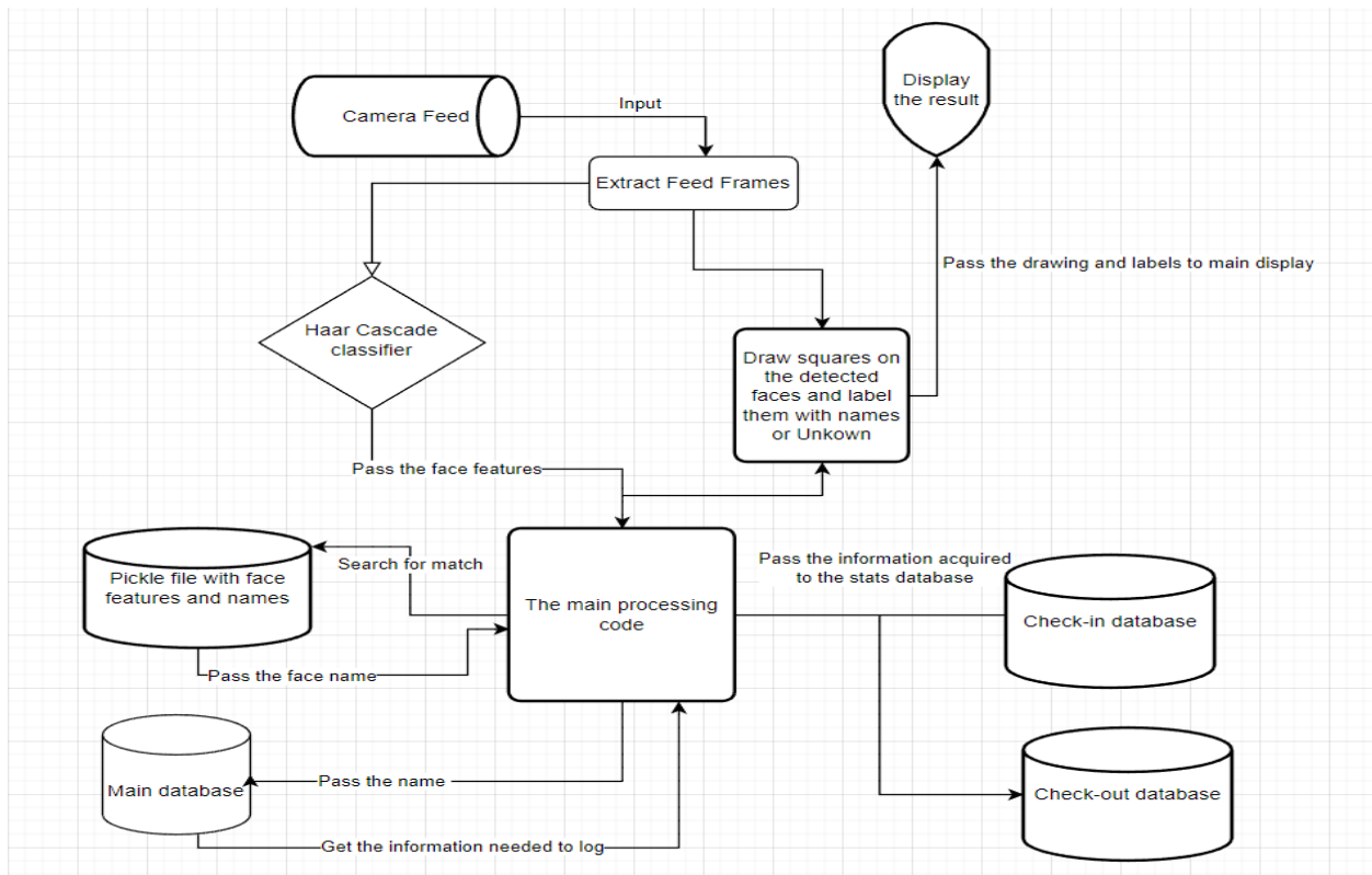
Fig. 8. Full system flow chart
