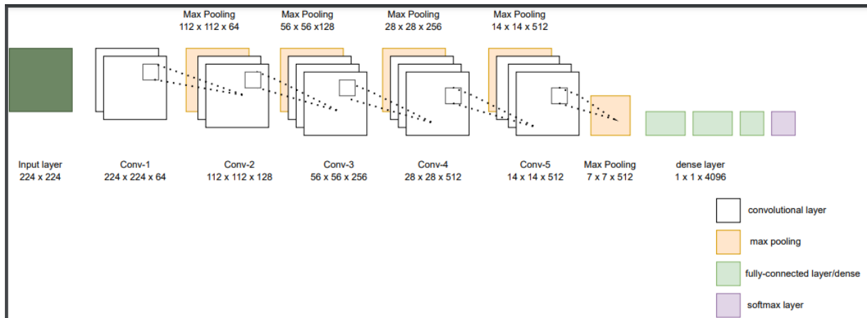
Fig. 3. An illustration of the architecture of the VGG-16 model
