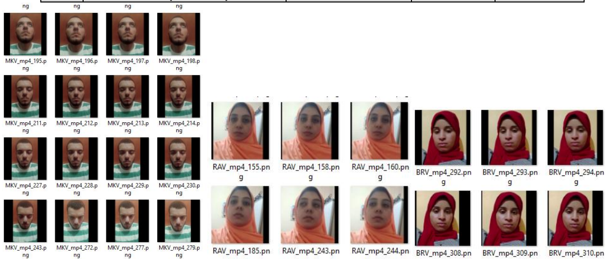
Fig. 6. Faces database.
